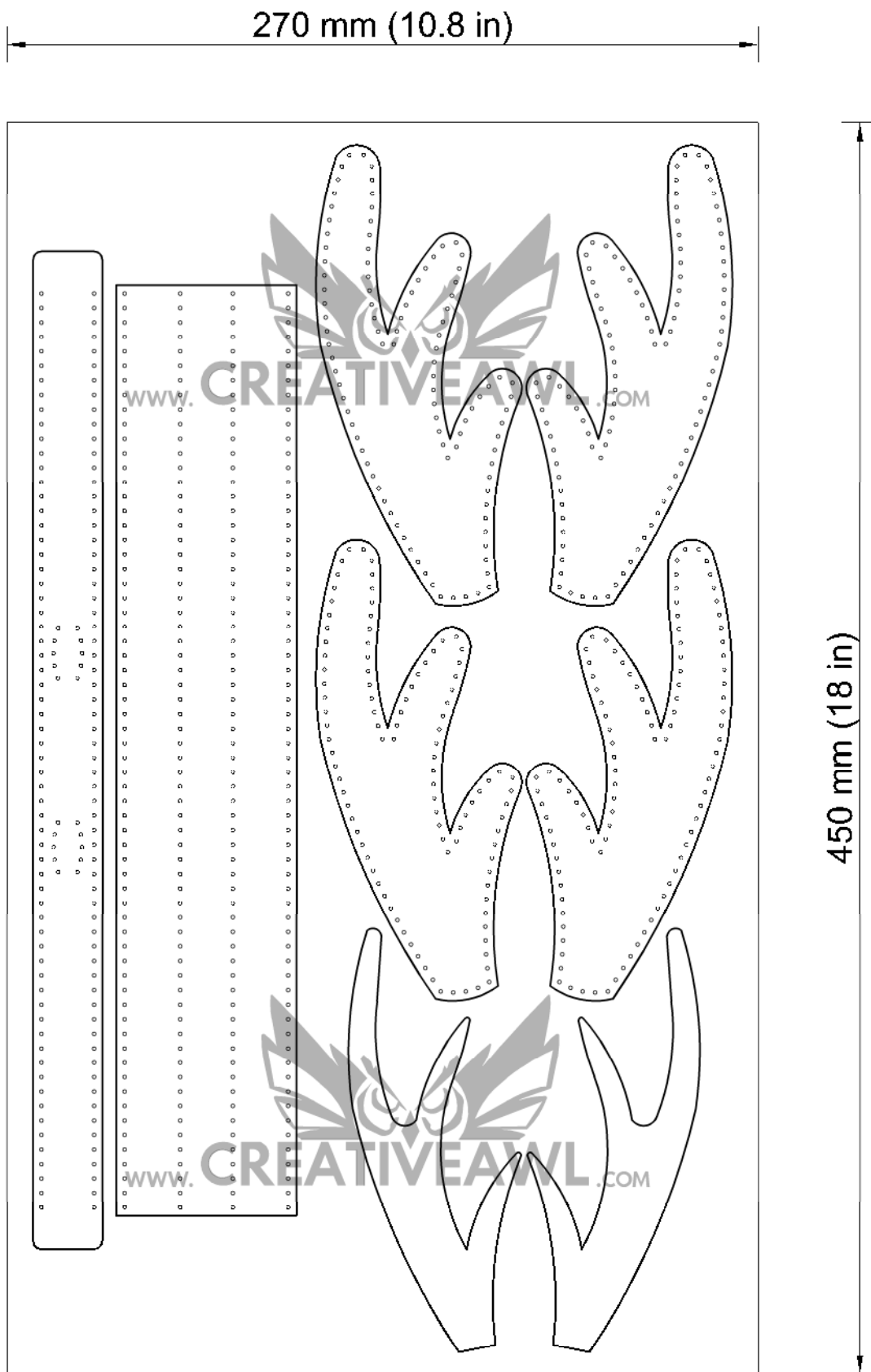
Sketch drawing Bill of materials
